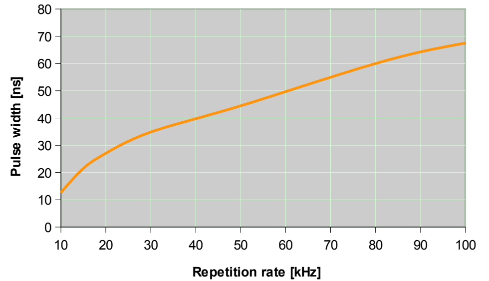
Sol 3W 532nm: Pulse Width
