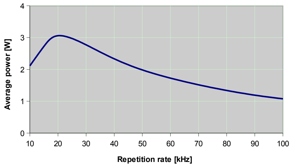
Sol 3W 532nm: Average Power
