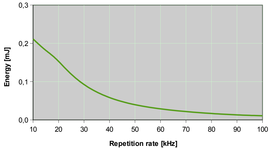
Sol 3W 532nm: Pulse Energy
