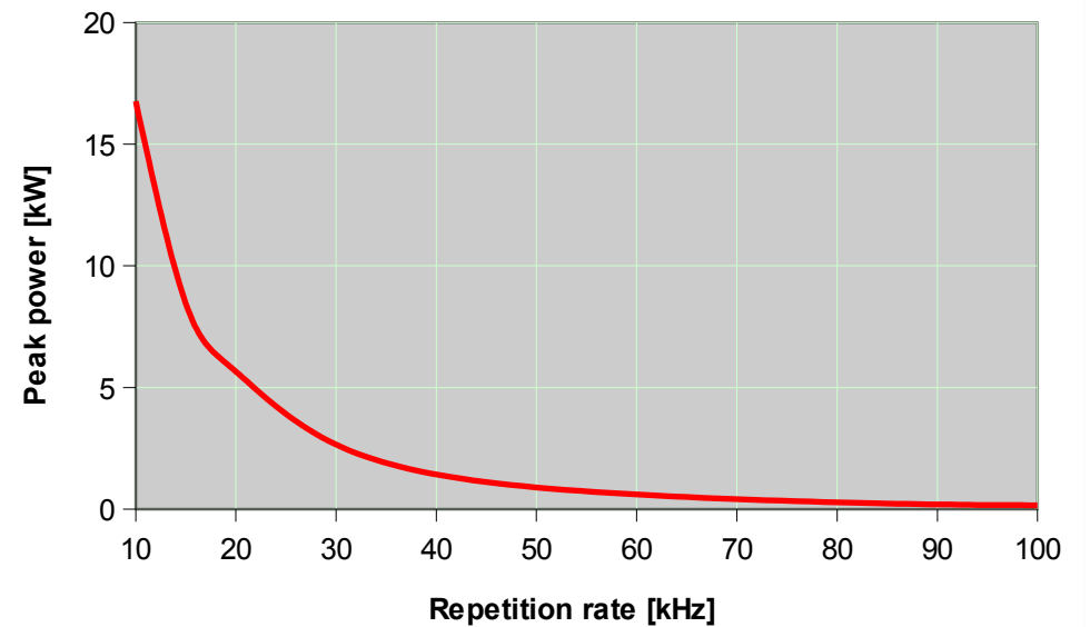
Sol 3W 532nm: Peak Power
